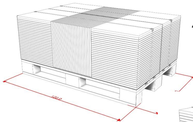
60 X 60 X 2 cm Product packaging
