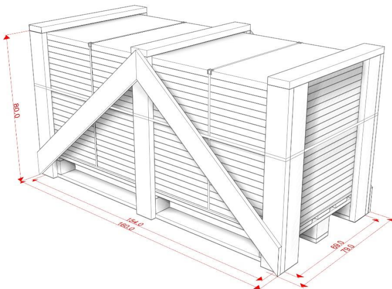
Slab products closed crate packaging
